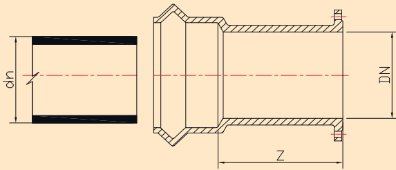
Flanged Socket
