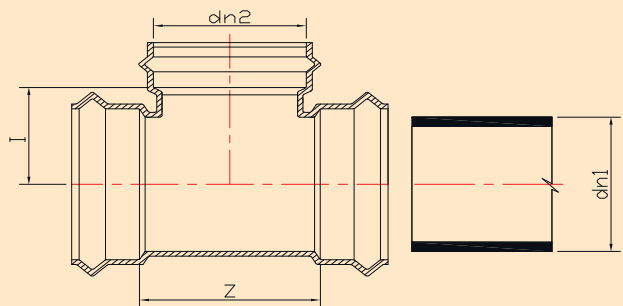
All Socket Tee
