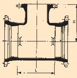
"K" TYPE
