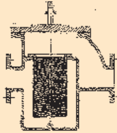
POT STRAINER
