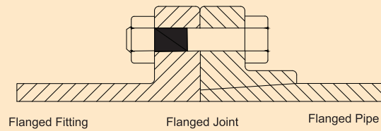
Flanged joint
