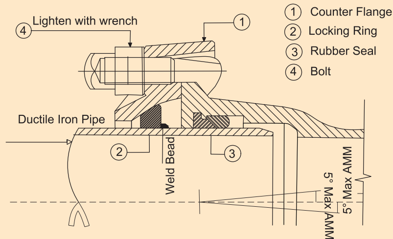
Restrained Joint
