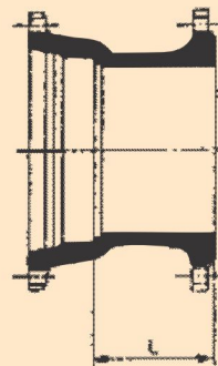
"K" TYPE
