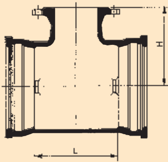
"T" TYPE
