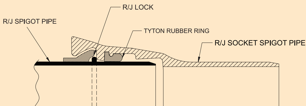
Double Chamber Retained Joint
