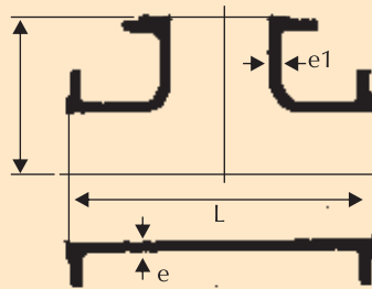
"I" TYPE
